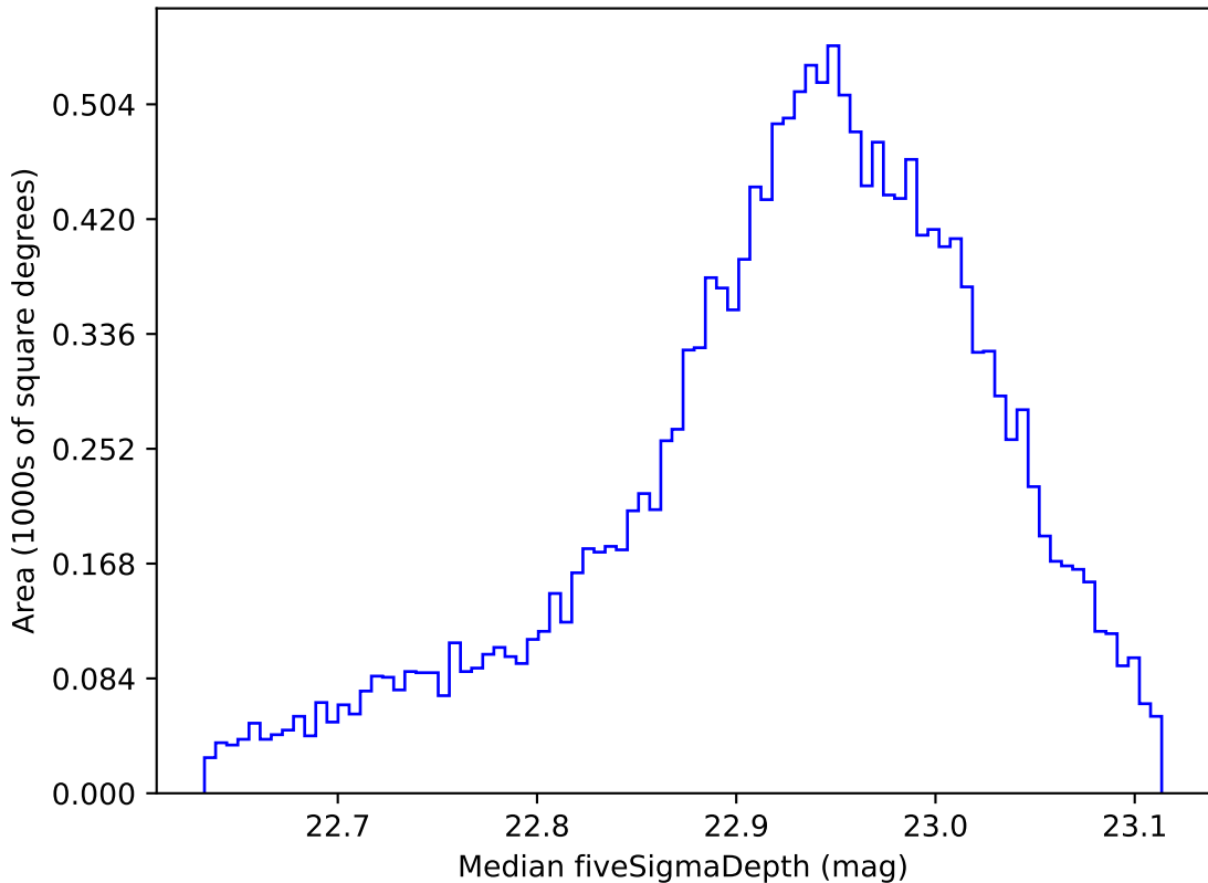
weather_cloudso16v3.4_10yrs WFD z band: Median fiveSigmaDepth
