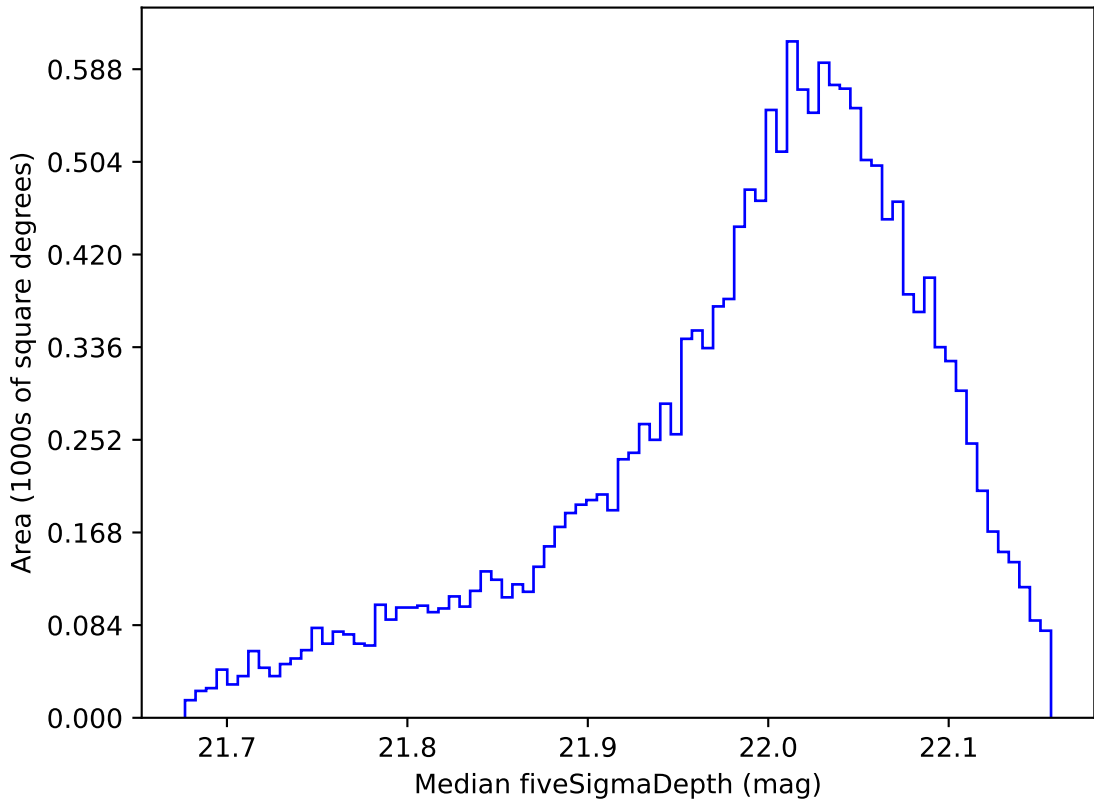
weather_cloudso16v3.4_10yrs WFD y band: Median fiveSigmaDepth
