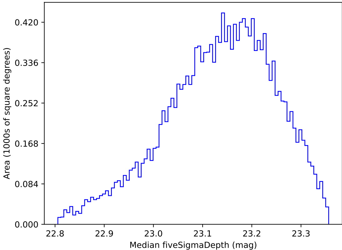
weather_cloudso16v3.4_10yrs WFD u band: Median fiveSigmaDepth
