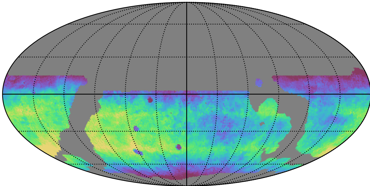
weather_cloudso16v3.4_10yrs WFD r band: Median fiveSigmaDepth
