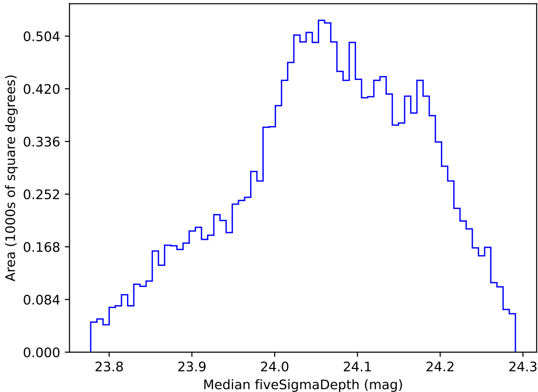
weather_cloudso16v3.4_10yrs WFD r band: Median fiveSigmaDepth
