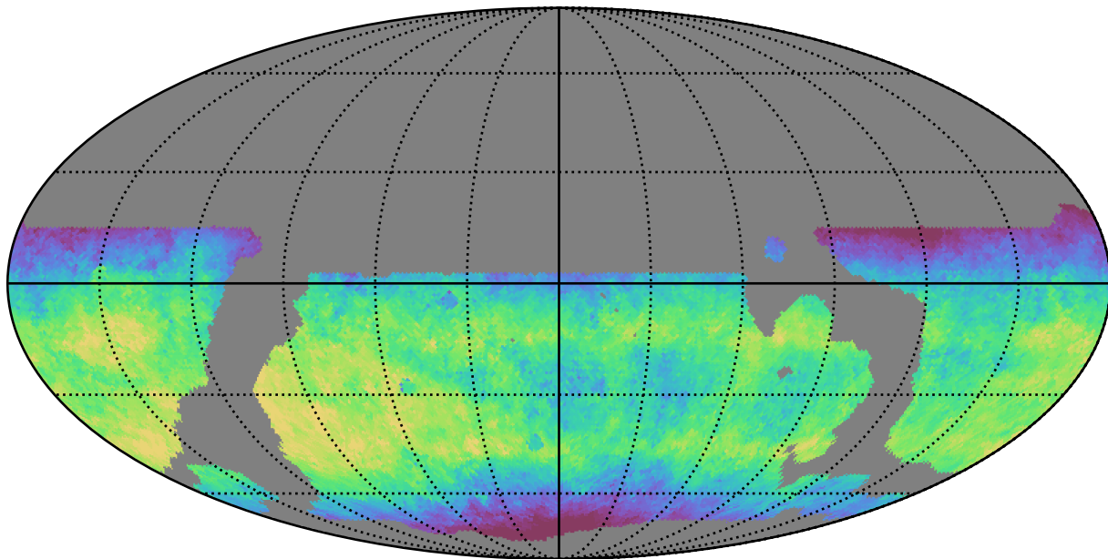
weather_cloudso16v3.4_10yrs WFD i band: Median fiveSigmaDepth
