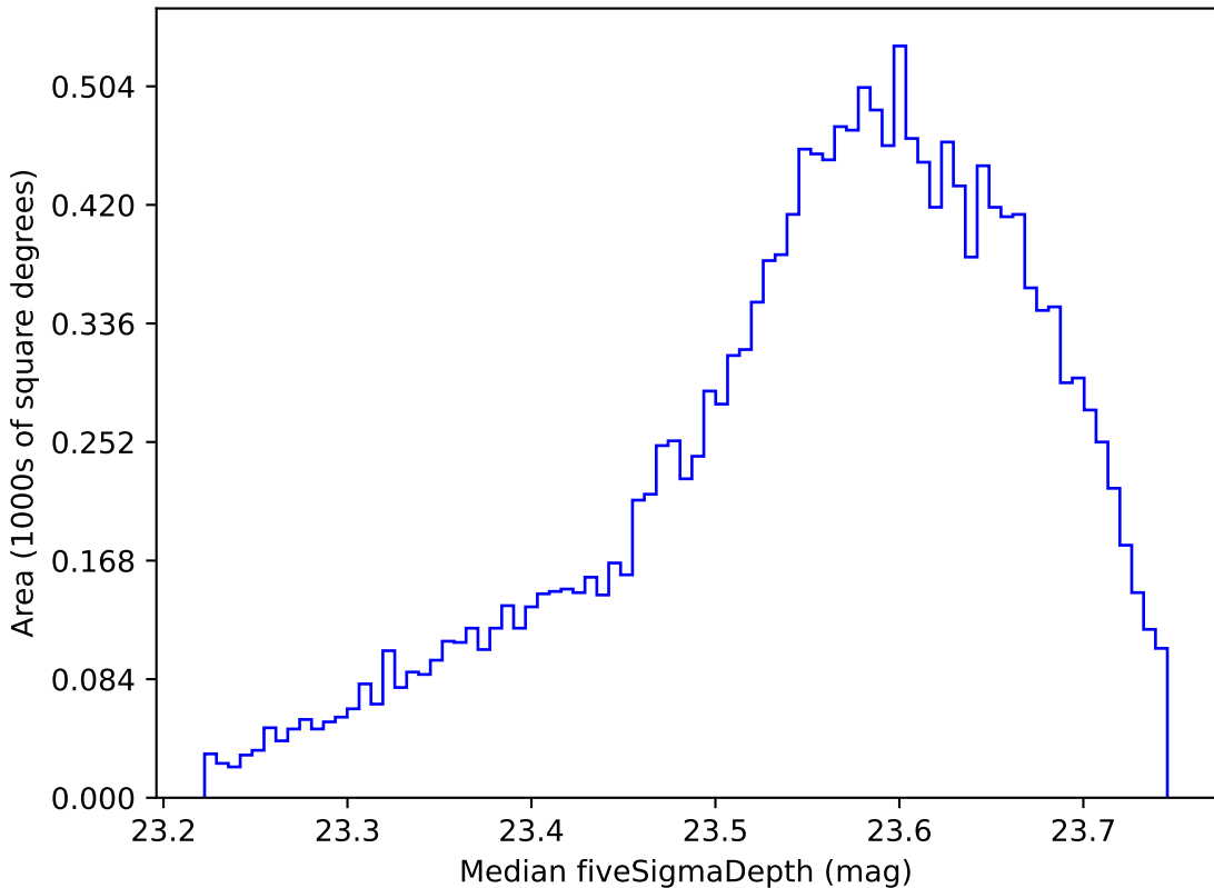
weather_cloudso16v3.4_10yrs WFD i band: Median fiveSigmaDepth
