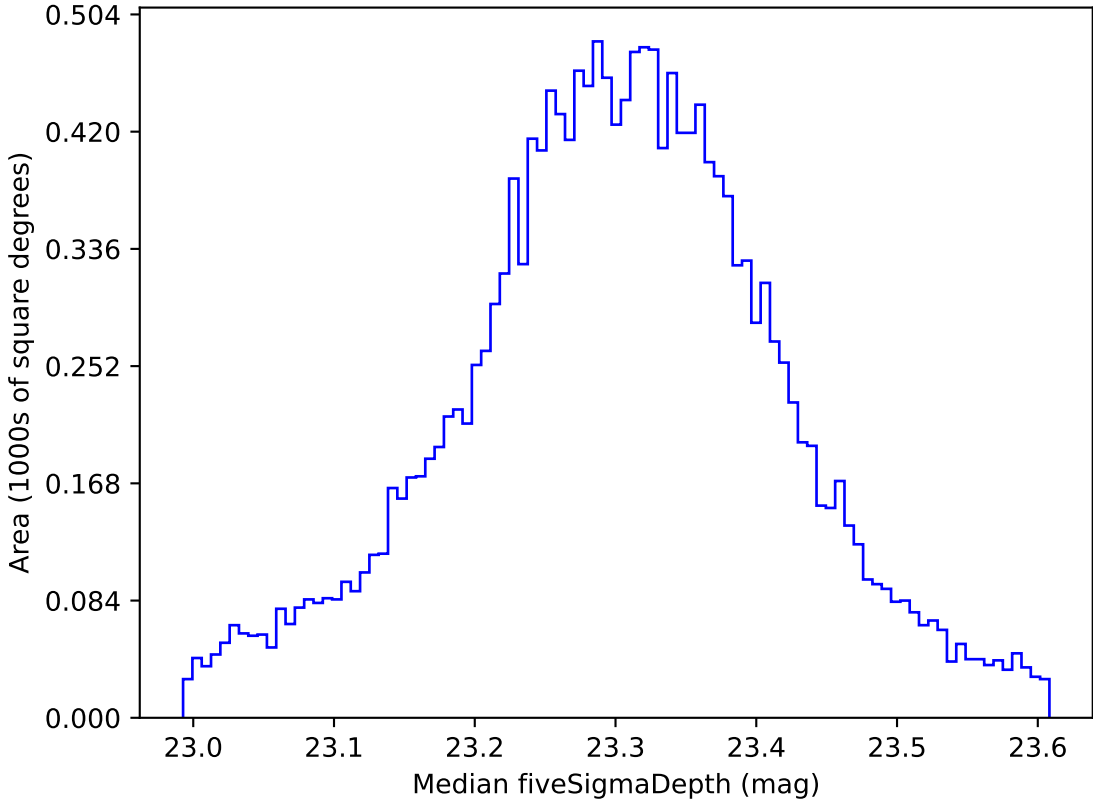
weather_cloudso16v3.4_10yrs WFD all bands: Median fiveSigmaDepth
