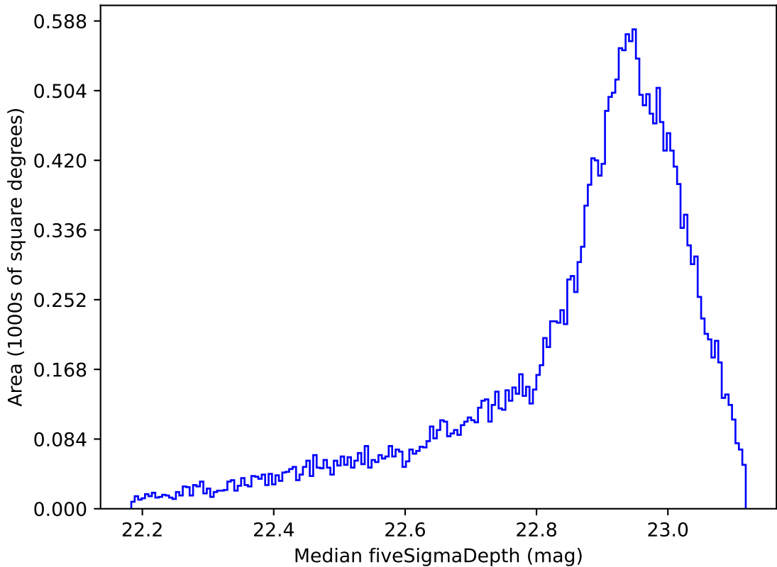
weather_cloudso16v3.4_10yrs All sky z band: Median fiveSigmaDepth
