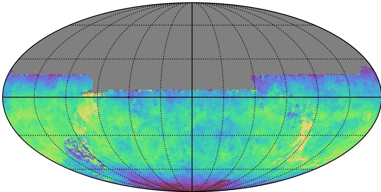
weather_cloudso16v3.4_10yrs All sky u band: Median fiveSigmaDepth
