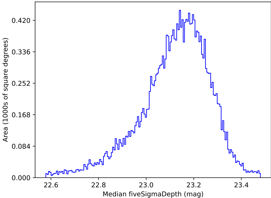
weather_cloudso16v3.4_10yrs All sky u band: Median fiveSigmaDepth
