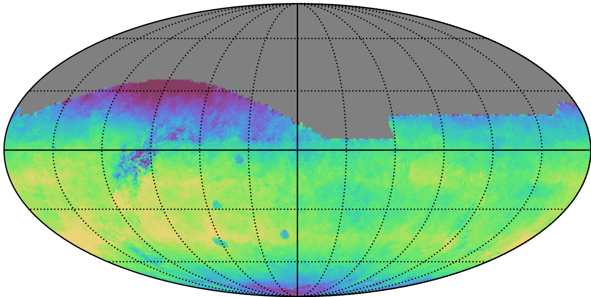
weather_cloudso16v3.4_10yrs All sky r band: Median fiveSigmaDepth
