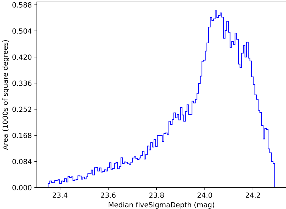
weather_cloudso16v3.4_10yrs All sky r band: Median fiveSigmaDepth
