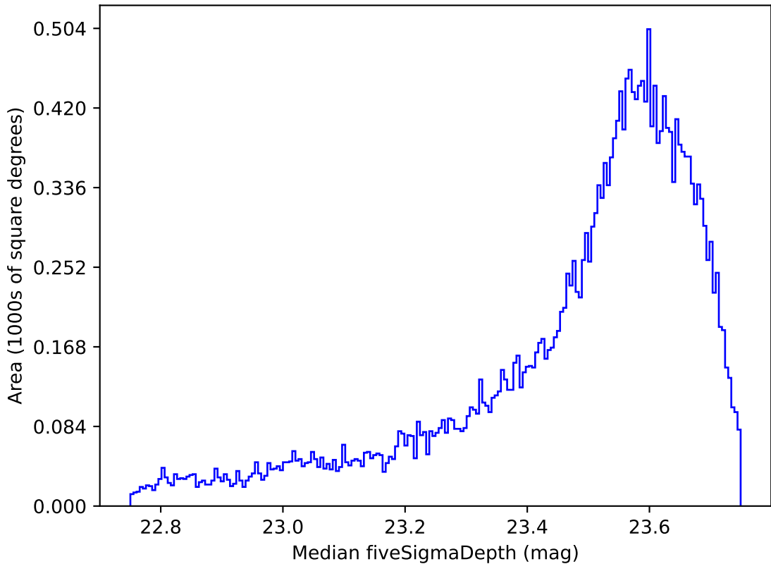
weather_cloudso16v3.4_10yrs All sky i band: Median fiveSigmaDepth
