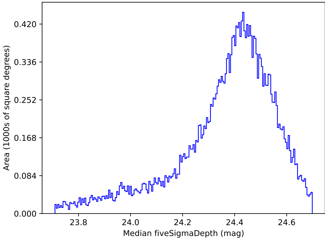
weather_cloudso16v3.4_10yrs All sky g band: Median fiveSigmaDepth
