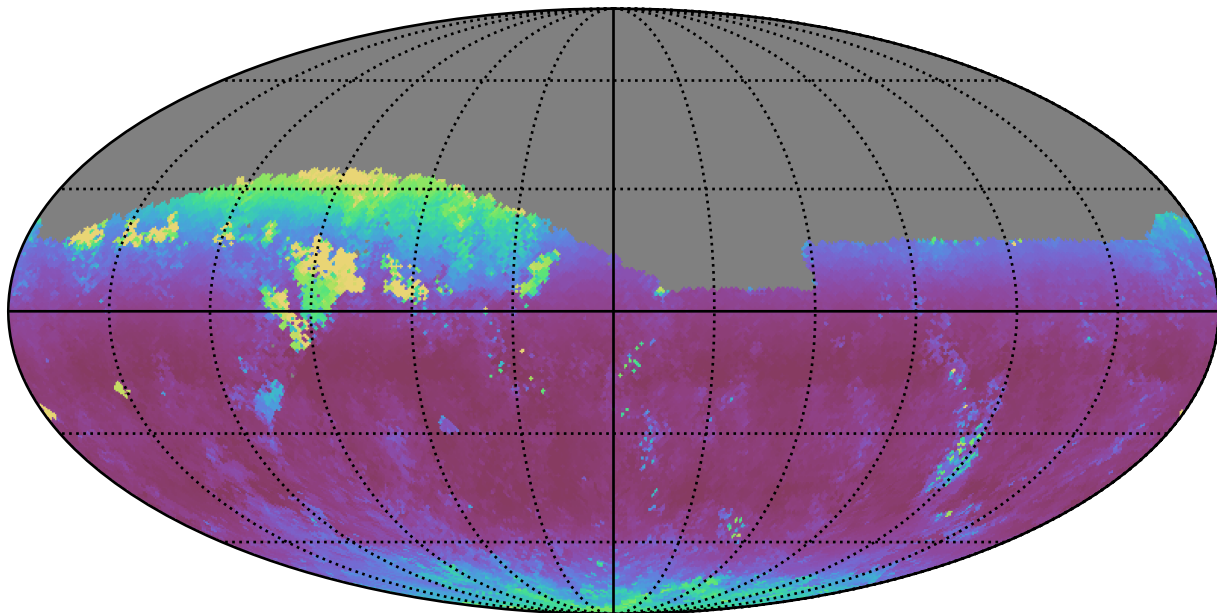
weather_cloudso16v3.4_10yrs Yr 1 z band: Median airmass
