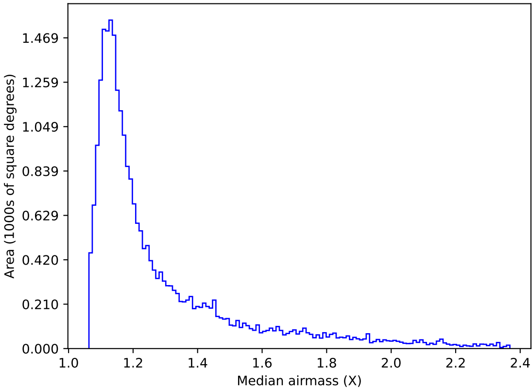
weather_cloudso16v3.4_10yrs Yr 1 z band: Median airmass
