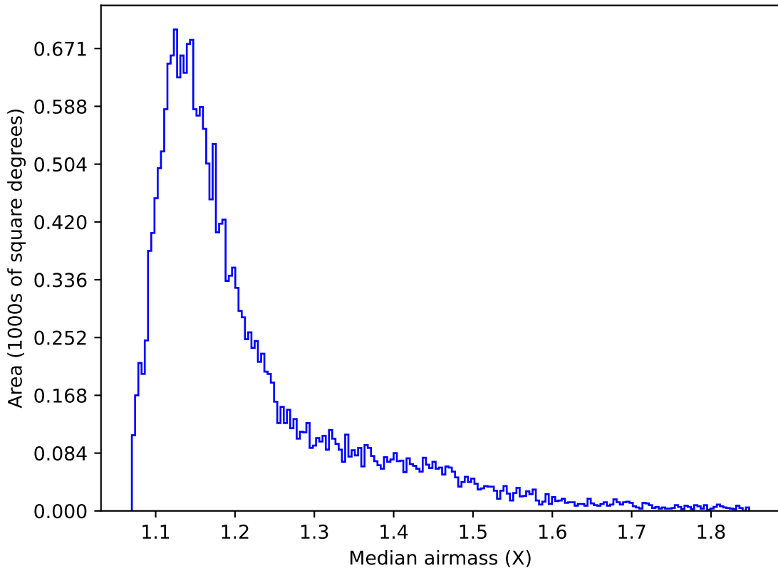
weather_cloudso16v3.4_10yrs Yr 1 y band: Median airmass
