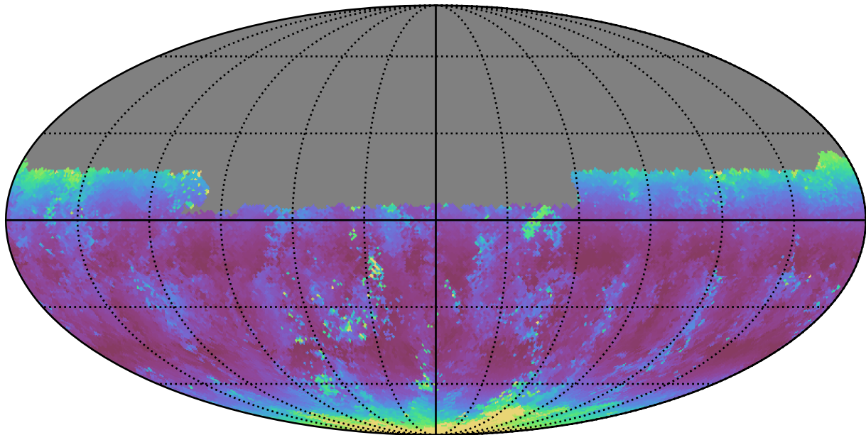
weather_cloudso16v3.4_10yrs Yr 1 u band: Median airmass
