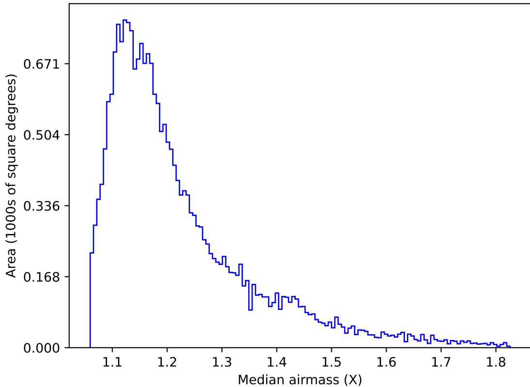
weather_cloudso16v3.4_10yrs Yr 1 u band: Median airmass
