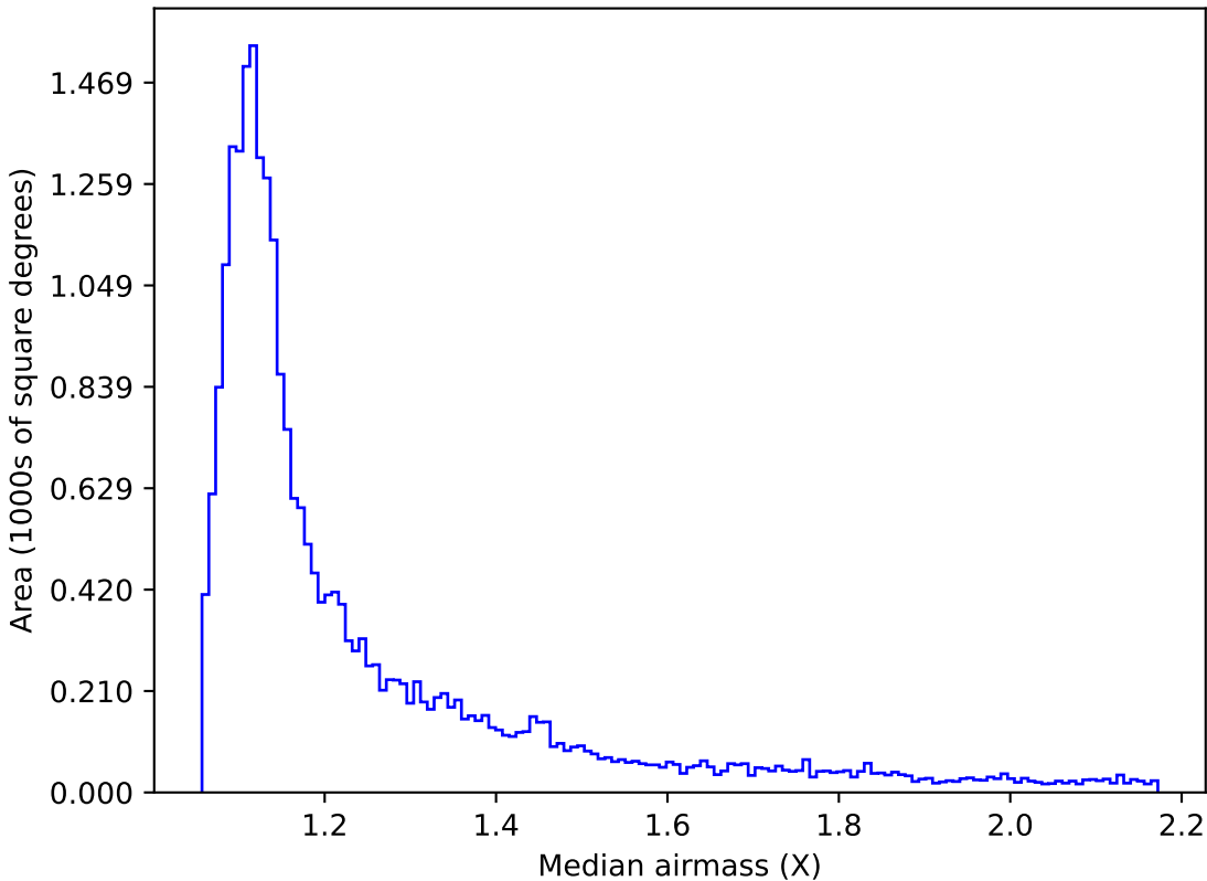
weather_cloudso16v3.4_10yrs Yr 1 r band: Median airmass
