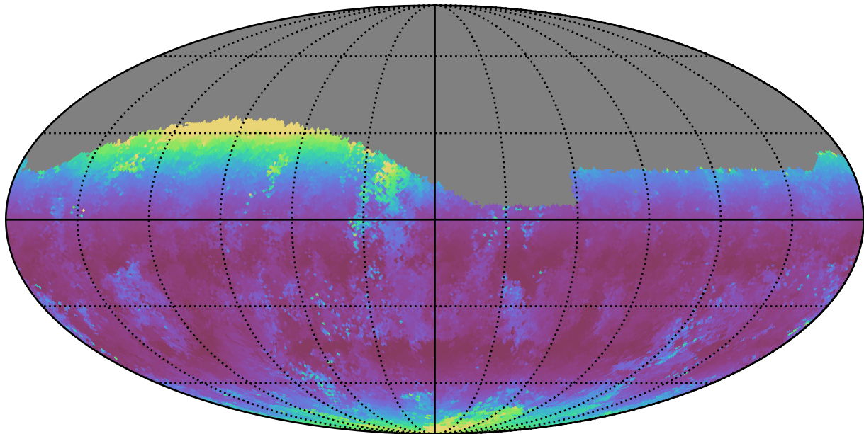
weather_cloudso16v3.4_10yrs Yr 1 g band: Median airmass
