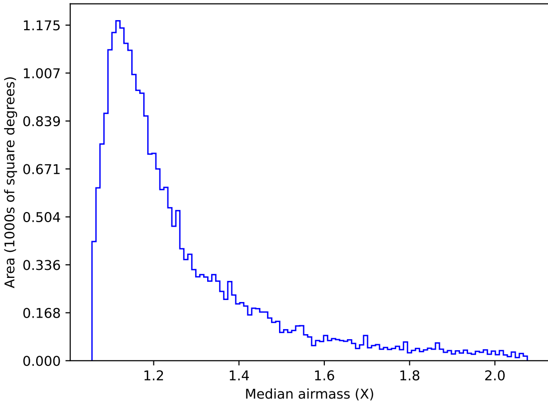
weather_cloudso16v3.4_10yrs Yr 1 g band: Median airmass
