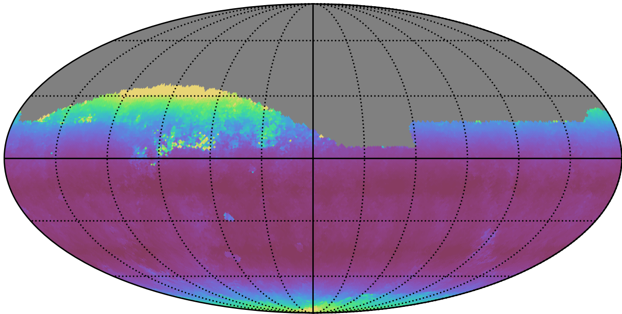
weather_cloudso16v3.4_10yrs Yr 1 all bands: Median airmass
