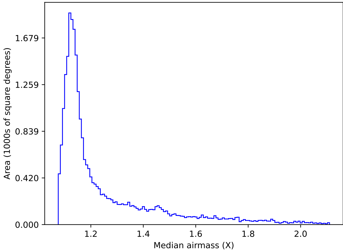
weather_cloudso16v3.4_10yrs Yr 1 all bands: Median airmass
