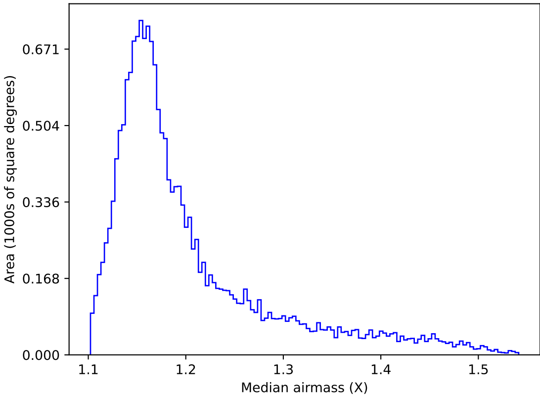
weather_cloudso16v3.4_10yrs WFD z band: Median airmass
