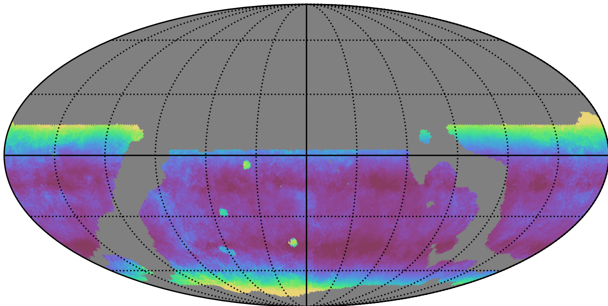
weather_cloudso16v3.4_10yrs WFD y band: Median airmass
