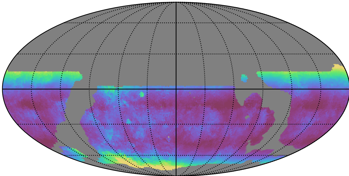
weather_cloudso16v3.4_10yrs WFD u band: Median airmass
