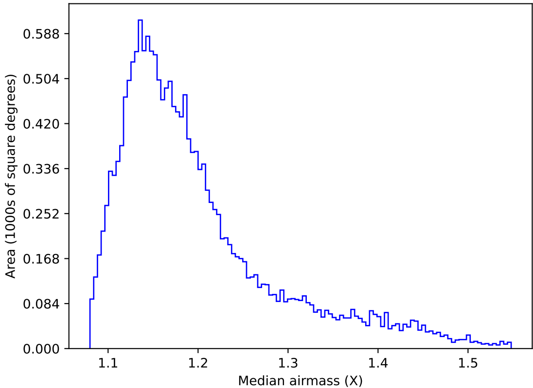
weather_cloudso16v3.4_10yrs WFD u band: Median airmass
