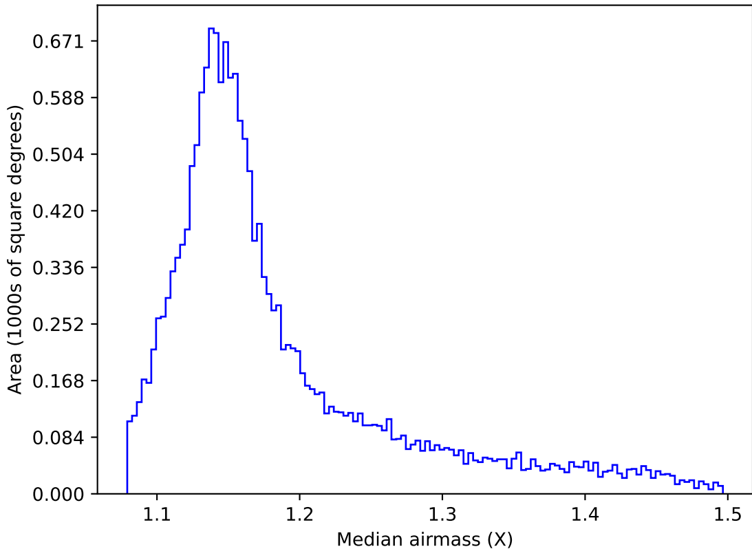
weather_cloudso16v3.4_10yrs WFD r band: Median airmass
