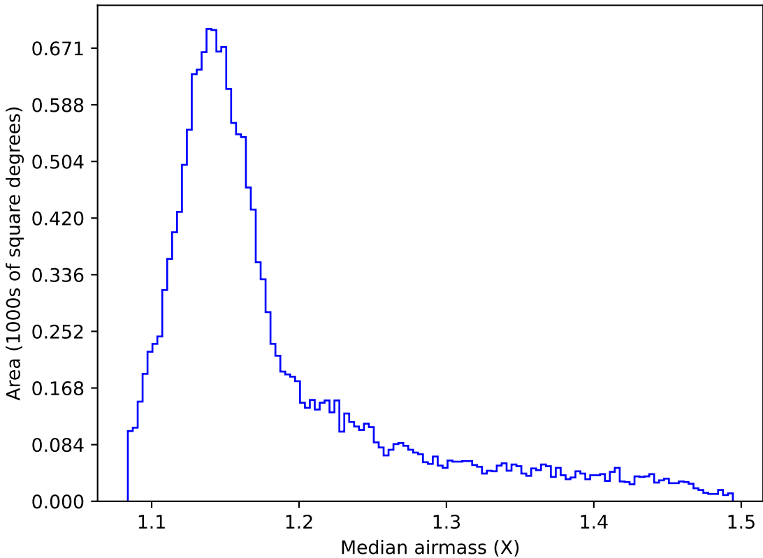
weather_cloudso16v3.4_10yrs WFD i band: Median airmass
