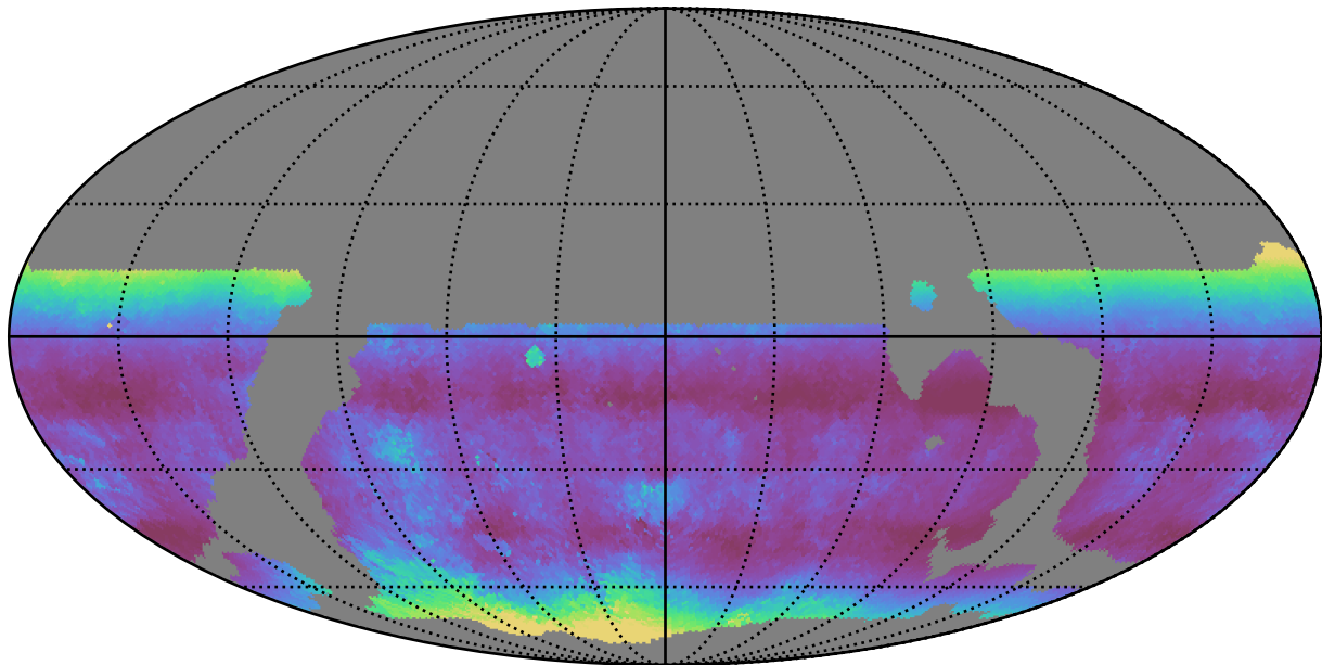
weather_cloudso16v3.4_10yrs WFD g band: Median airmass
