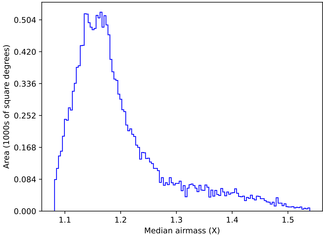
weather_cloudso16v3.4_10yrs WFD g band: Median airmass
