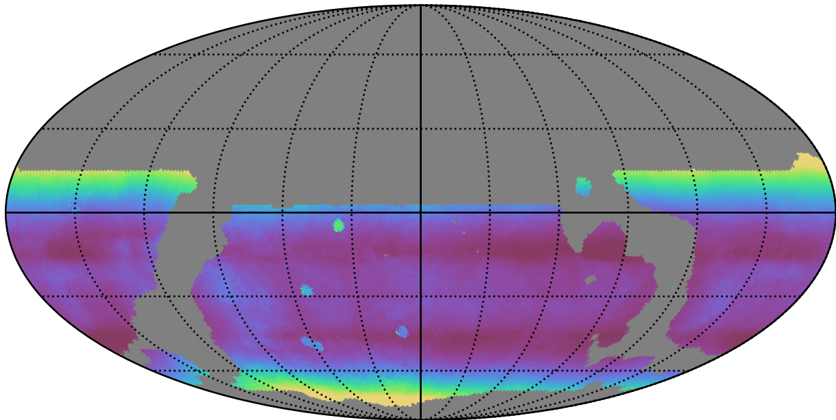
weather_cloudso16v3.4_10yrs WFD all bands: Median airmass
