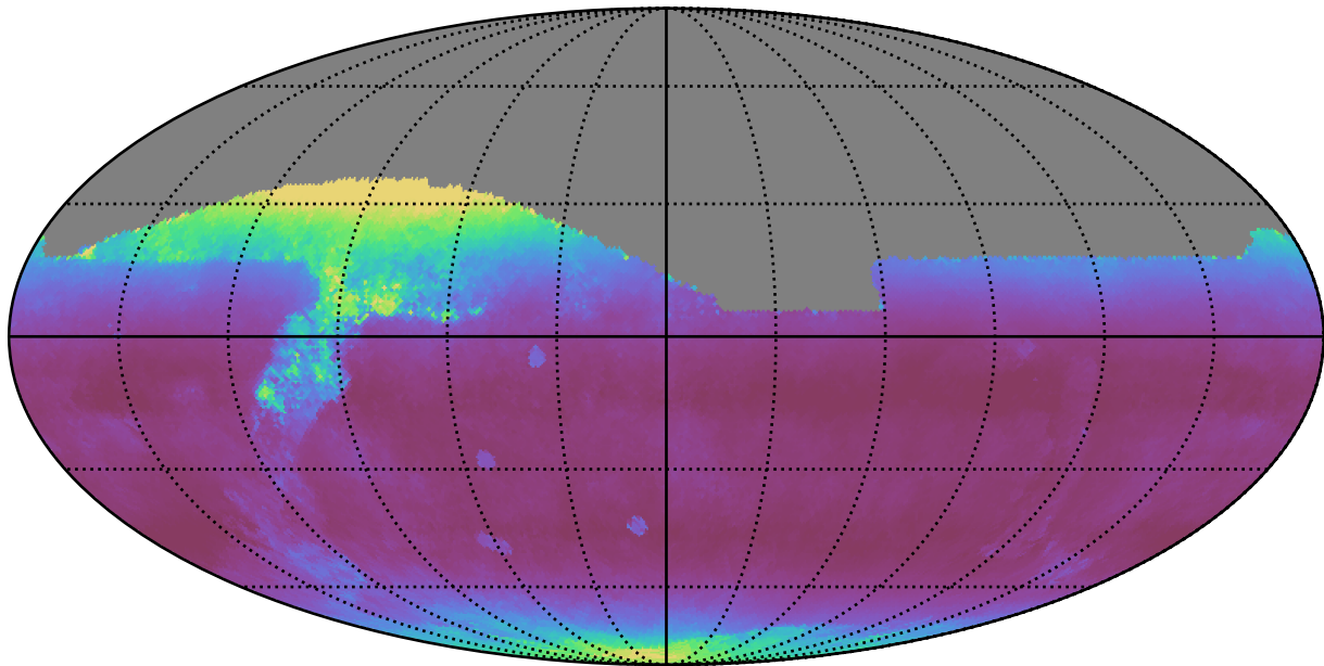
weather_cloudso16v3.4_10yrs All sky z band: Median airmass
