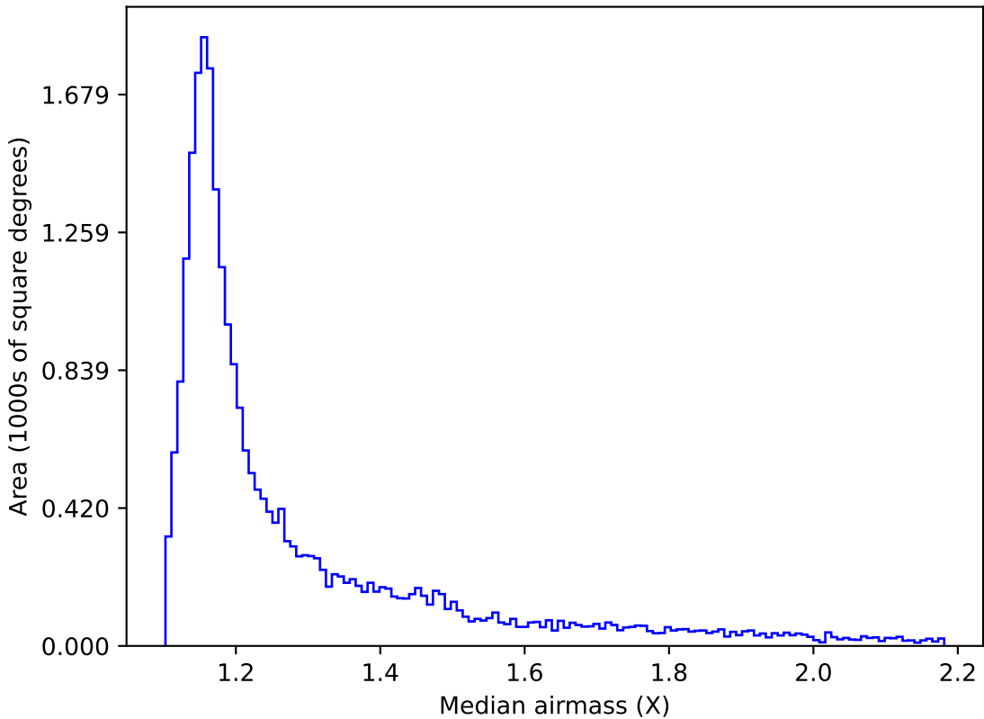
weather_cloudso16v3.4_10yrs All sky z band: Median airmass
