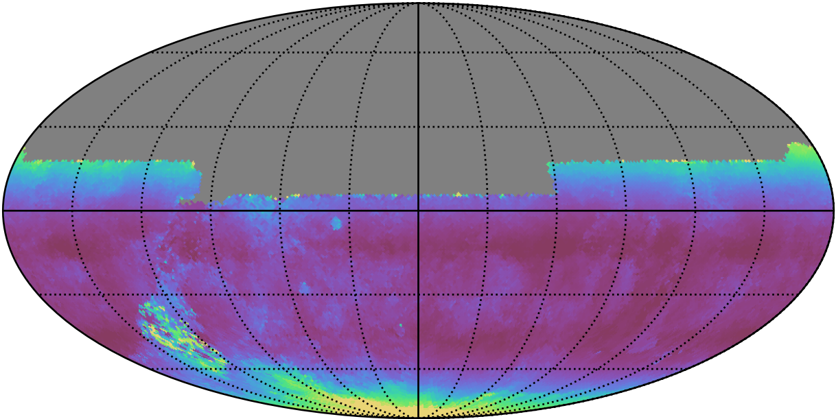
weather_cloudso16v3.4_10yrs All sky u band: Median airmass
