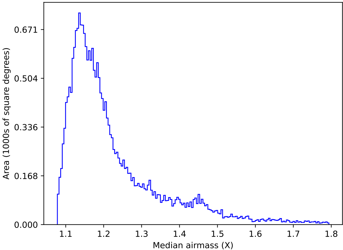
weather_cloudso16v3.4_10yrs All sky u band: Median airmass
