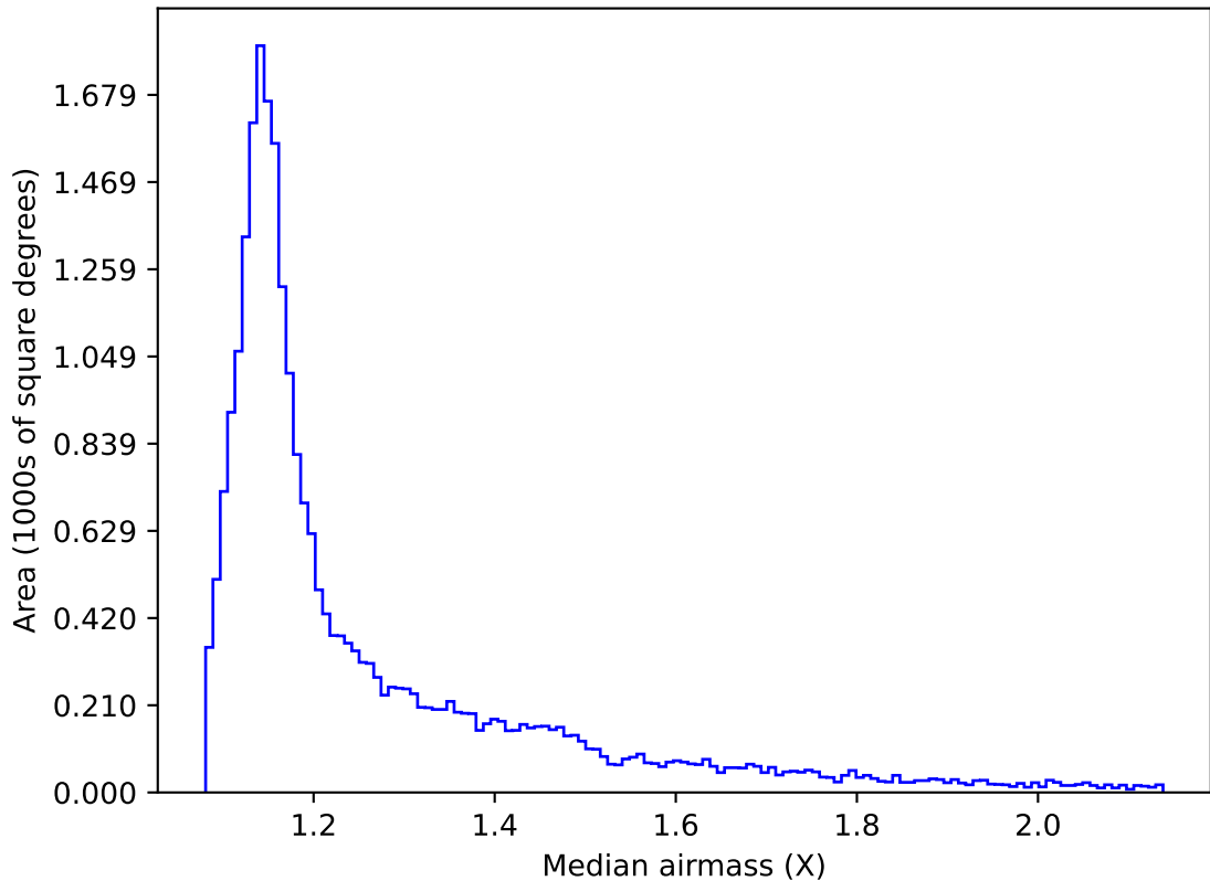
weather_cloudso16v3.4_10yrs All sky r band: Median airmass
