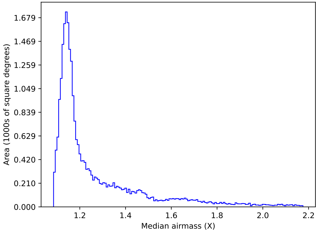
weather_cloudso16v3.4_10yrs All sky i band: Median airmass
