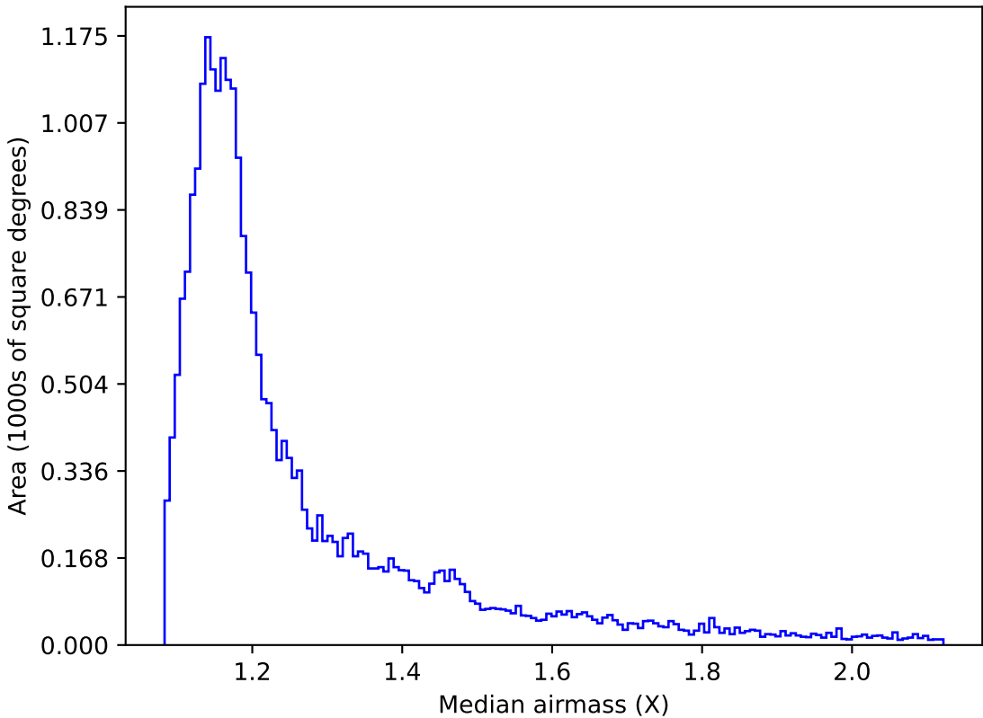
weather_cloudso16v3.4_10yrs All sky g band: Median airmass
