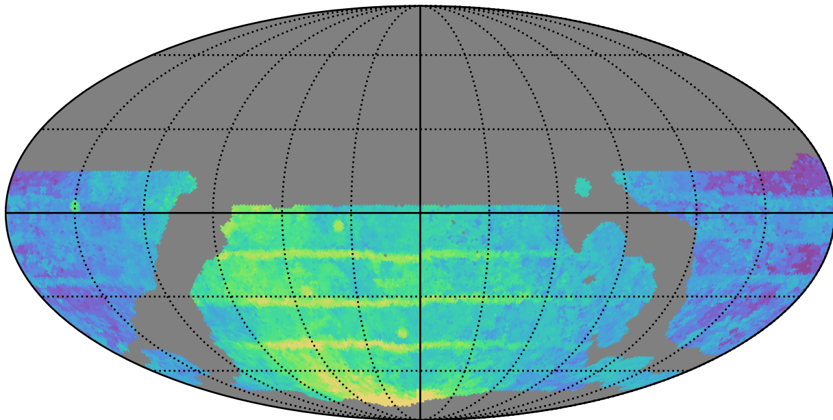
weather_cloudso16v3.4_10yrs WFD z band: Median Season Length
