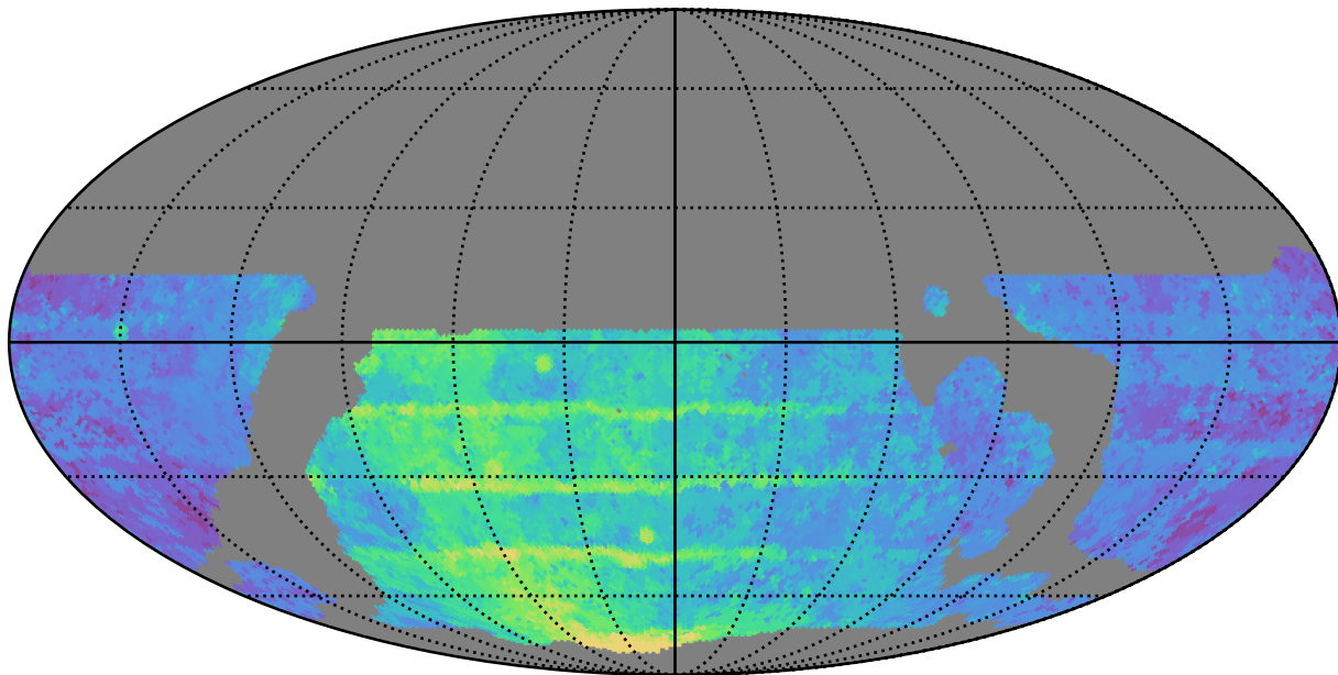
weather_cloudso16v3.4_10yrs WFD y band: Median Season Length
