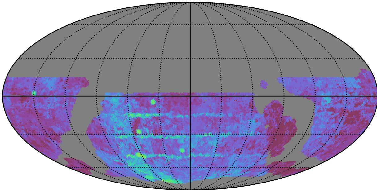
weather_cloudso16v3.4_10yrs WFD u band: Median Season Length
