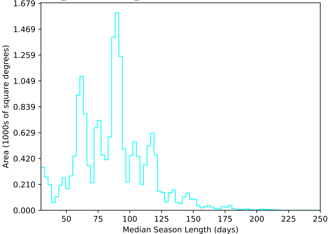
weather_cloudso16v3.4_10yrs WFD u band: Median Season Length
