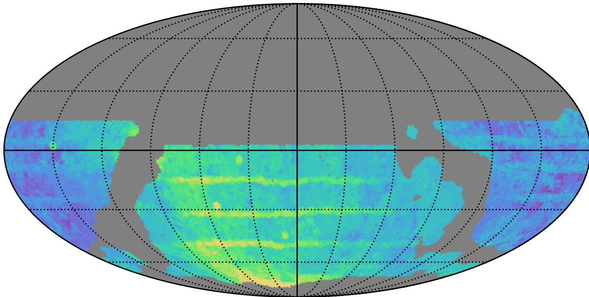
weather_cloudso16v3.4_10yrs WFD r band: Median Season Length
