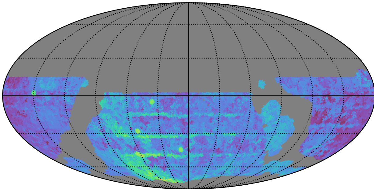
weather_cloudso16v3.4_10yrs WFD g band: Median Season Length
