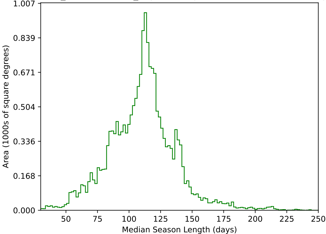
weather_cloudso16v3.4_10yrs WFD g band: Median Season Length
