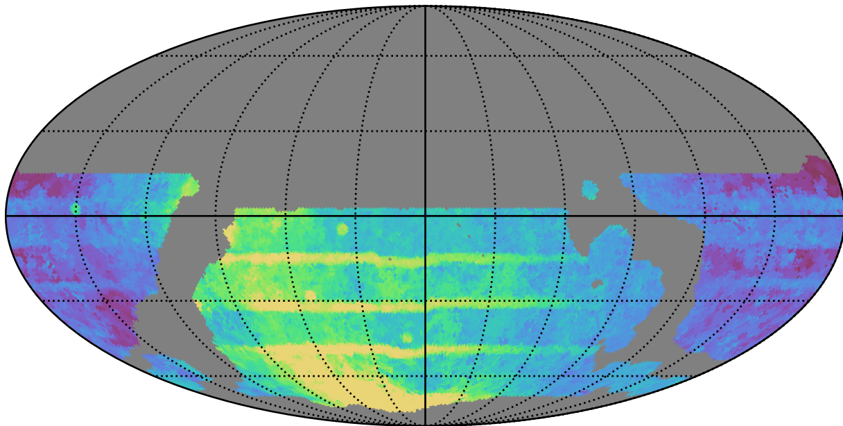
weather_cloudso16v3.4_10yrs WFD all bands: Median Season Length
