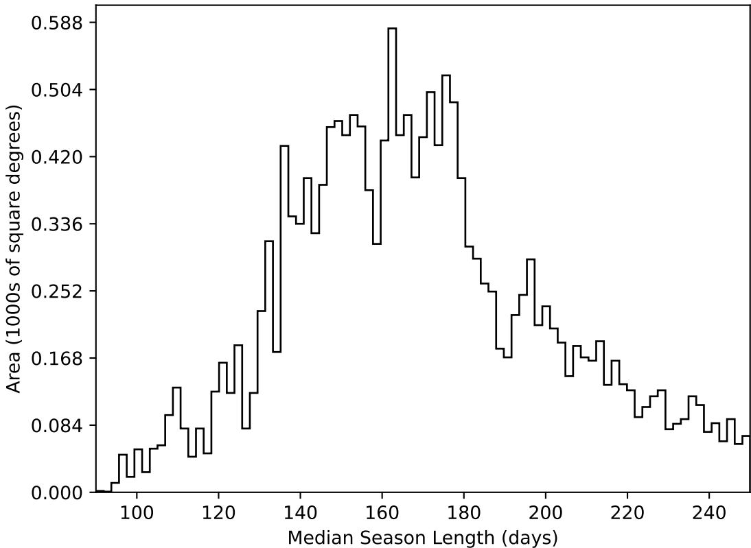
weather_cloudso16v3.4_10yrs WFD all bands: Median Season Length
